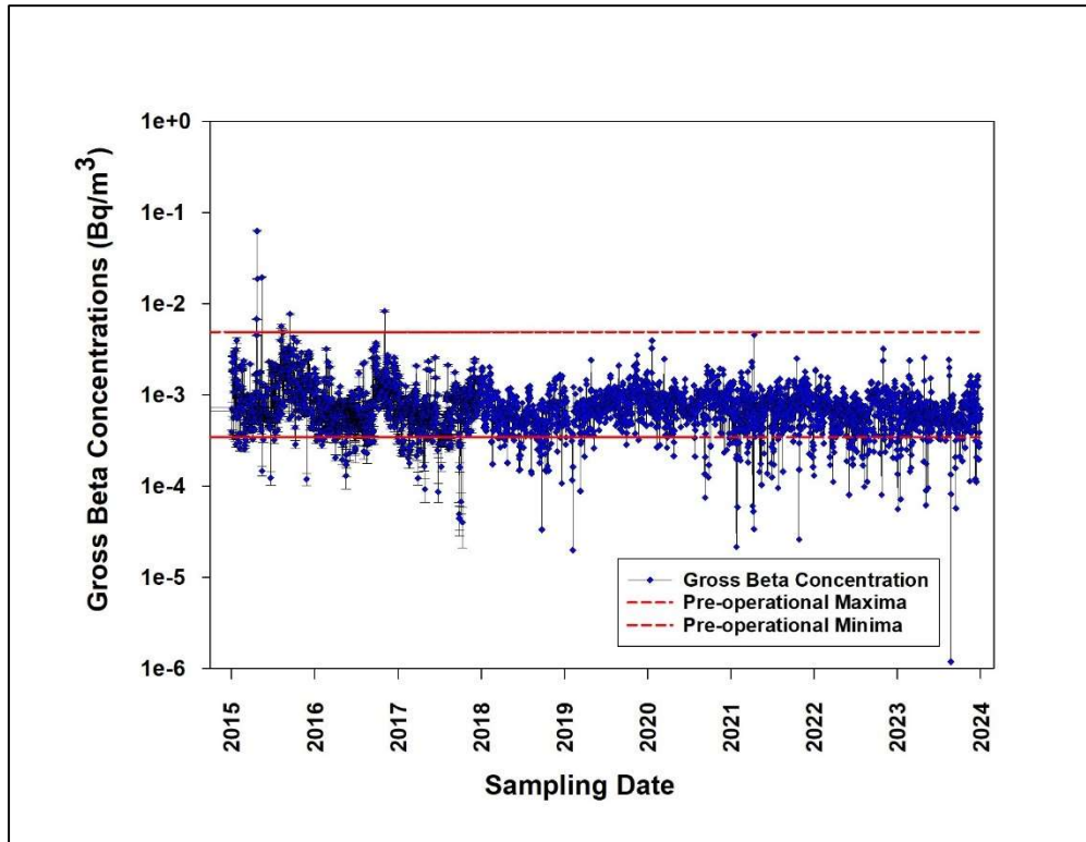
Figure 2.9. Gross Beta Concentrations at Station A during 2015-2023
