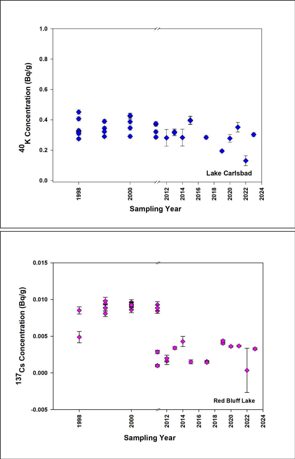
Figure 7.8. Historical Concentration of ^{137}\text{Cs} and ^{40}\text{K} in Sediment Samples in Three Regional Reservoirs
