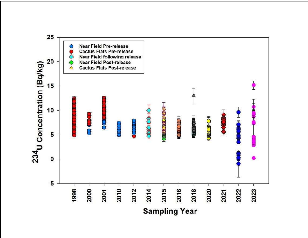
Figure 4.5. Historical Concentrations of 238 U and 234 U in WIPP Soil
