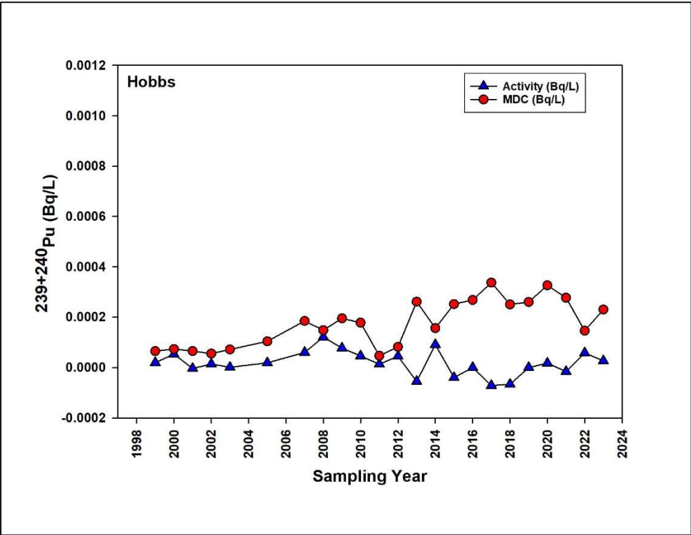
Figure 6.4. 238 Pu and 239+240 Pu Concentrations in Hobbs Drinking Water
