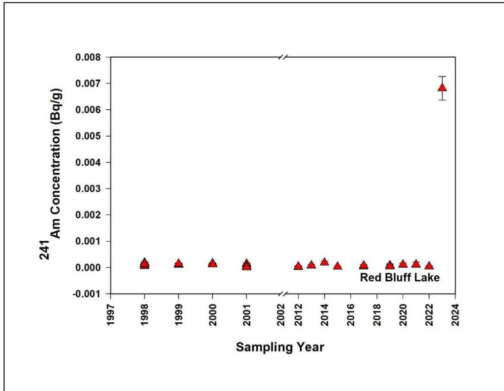
Figure 7.4. Historical Concentrations of ^{241}\text{Am} in Regional Reservoir Sediments
