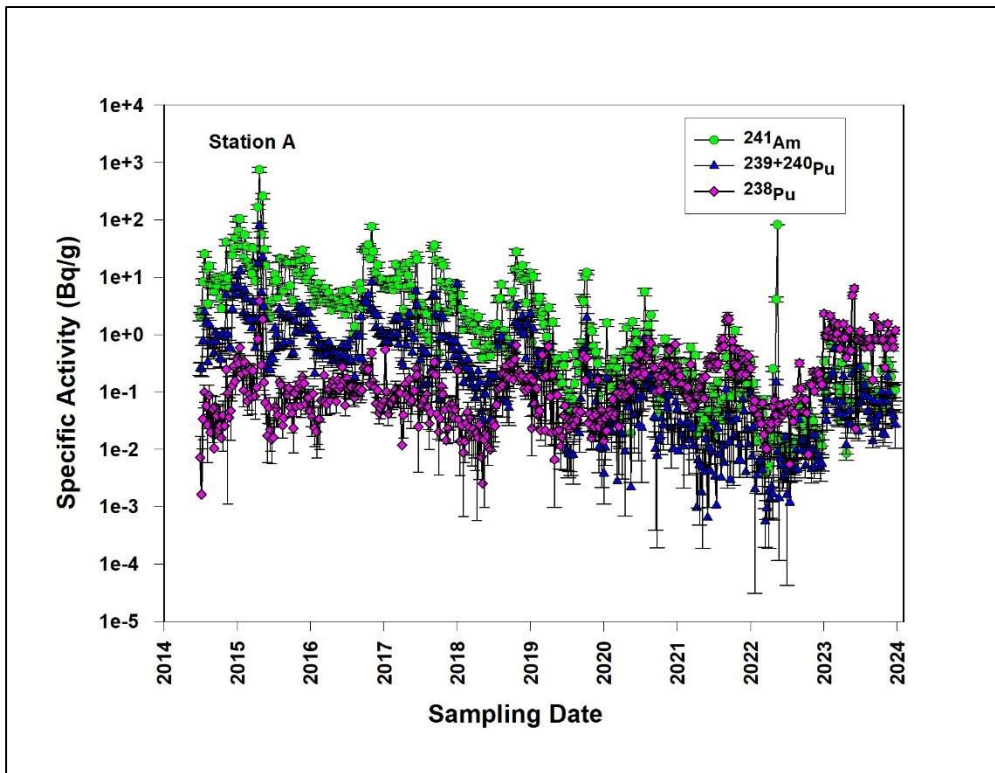
Figure 2.11. Weekly Specific Activities of 241 Am, 239+240 Pu, and 238 Pu at Station A
