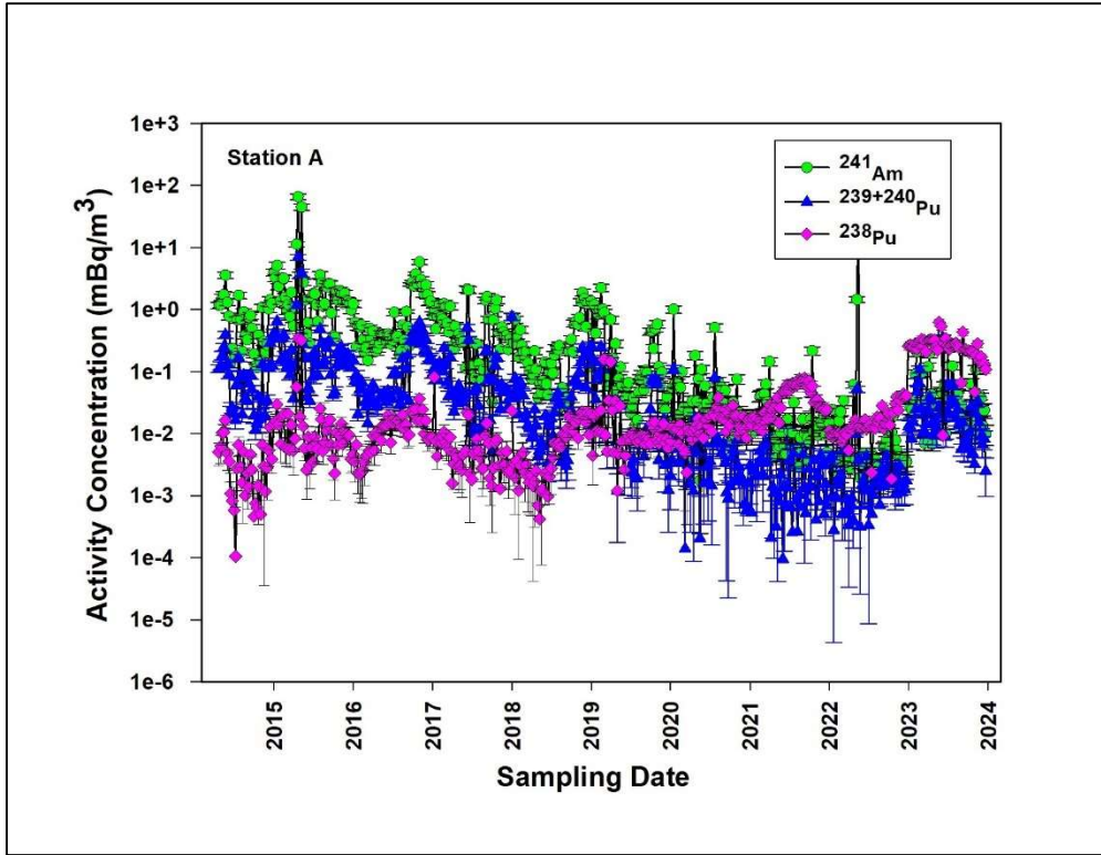
Figure 2.10. Weekly Concentrations of 241 Am, 239+240 Pu, and 238 Pu at Station A
