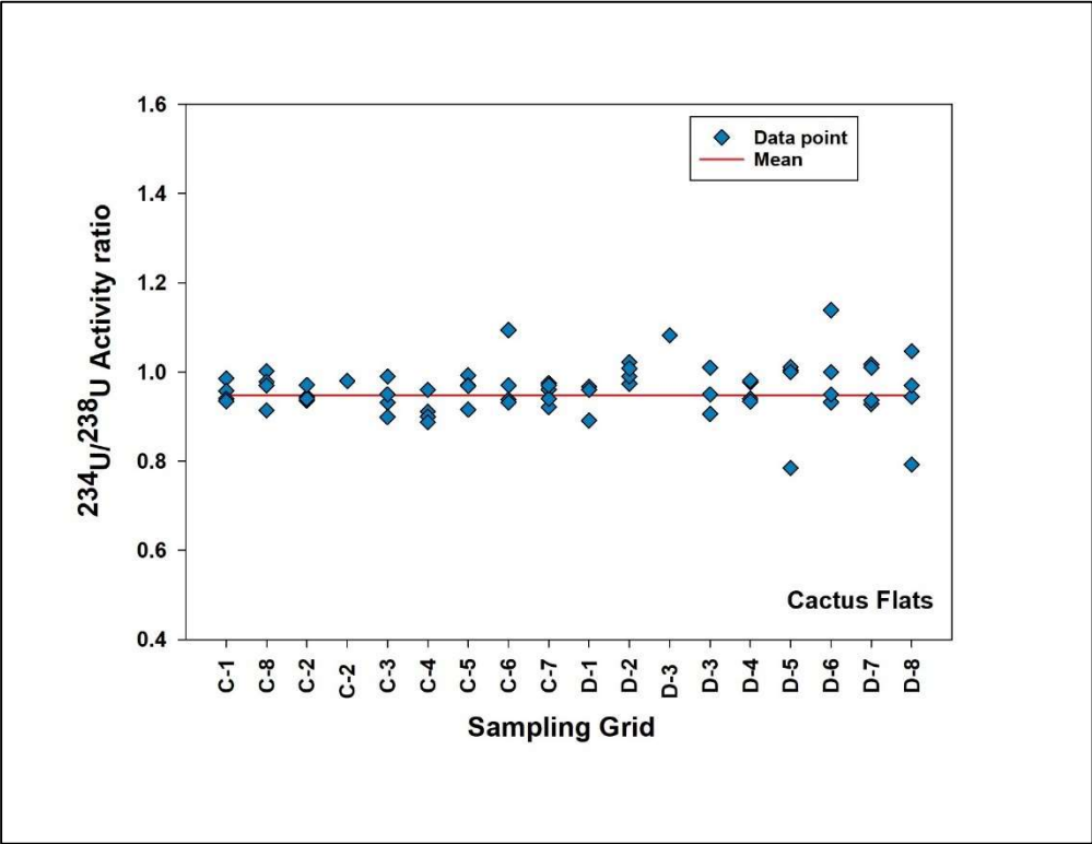
Figure 4.6. The ^{234}\text{U}/^{238}\text{U} Activity Ratio in WIPP Soil During 2015-2023
