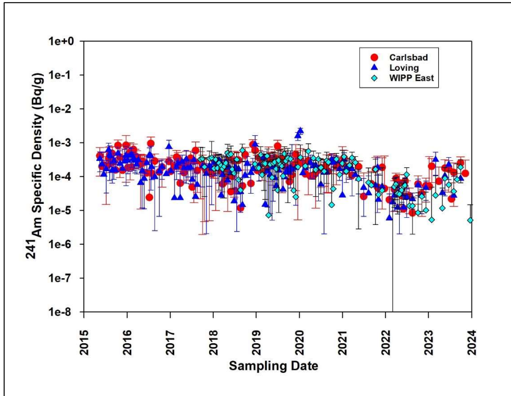
Figure 3.7. Historical 239+240 Pu (top) and 241 Am (bottom) Specific Activities at the Carlsbad, Loving, and WIPP East Stations
