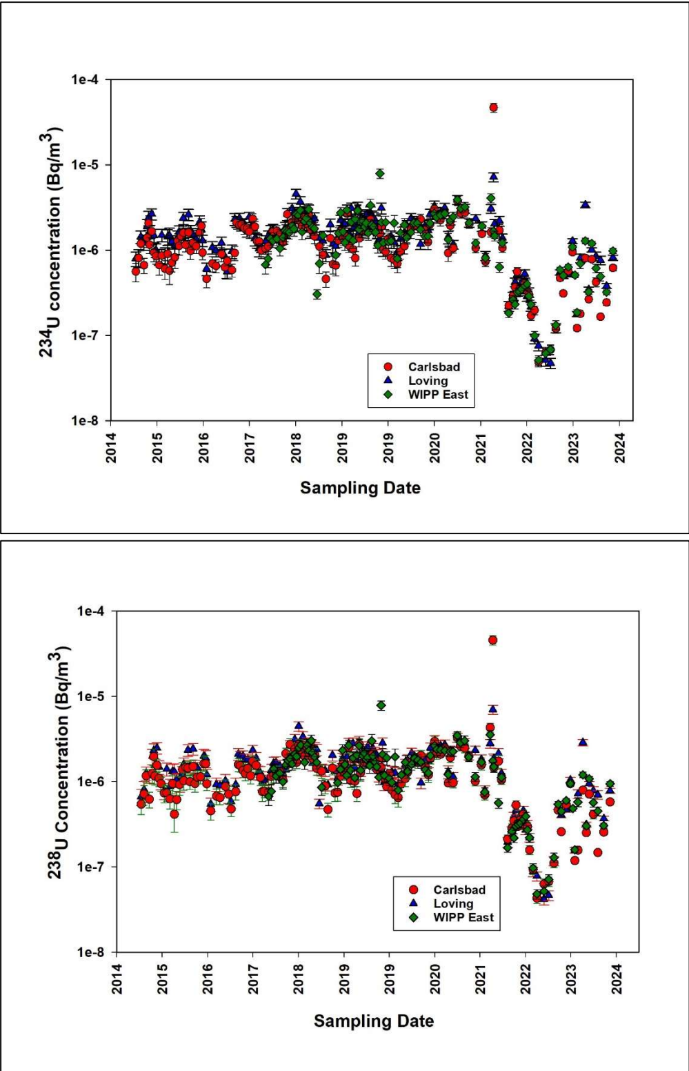
Figure 3.9. ^{234}\text{U} and ^{238}\text{U} Concentrations at the Carlsbad, Loving, and WIPP East Stations
