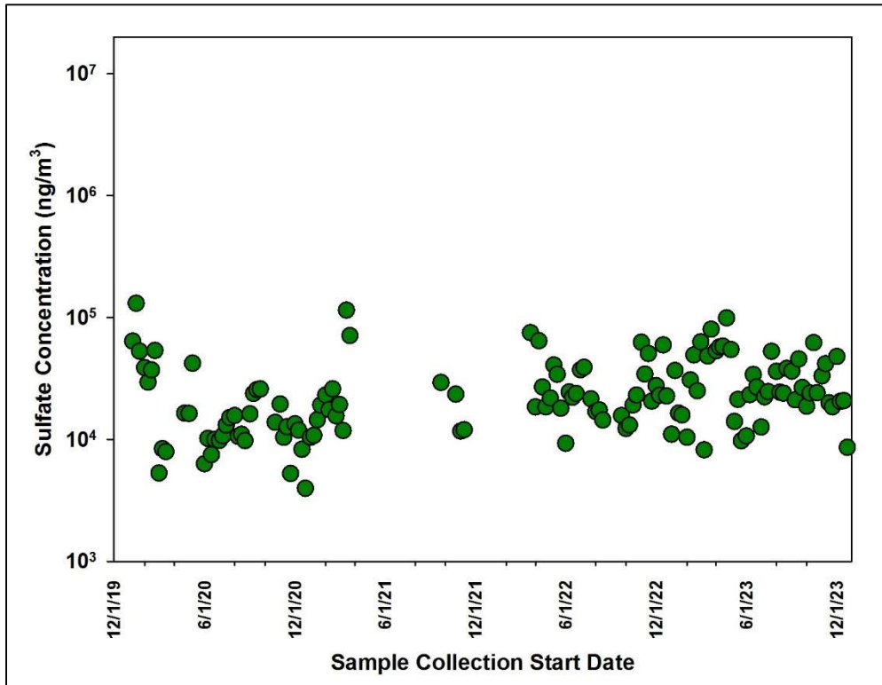
Figure 10.1. Historical Concentrations of Selected Inorganic Anions at Station A
