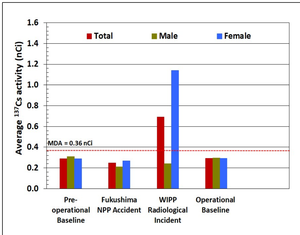
Figure 9.7. Average ^{137}\text{Cs} activity (nCi) among LDBC participants during 1997-2023
