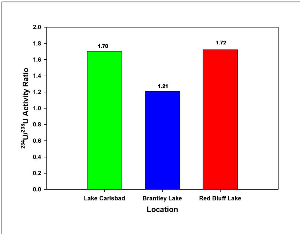
Figure 7.6. The ^{234}\text{U}/^{238}\text{U} Activity Ratio in Sediment Samples in Three Regional Reservoirs in 2023
